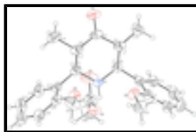
Fig. 1. Perspective view of the molecule showing the anisotropic displacement ellipsoids at 30% probability level.
