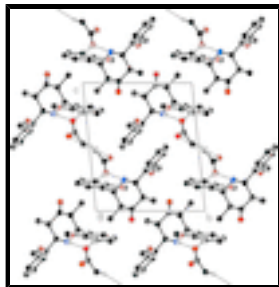
Fig. 2. The crystal packing of the molecules viewed down a -axis. For clarity, hydrogen atoms which are not involved in hydrogen bonding are omitted
